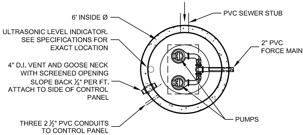
Pump Station Plan
